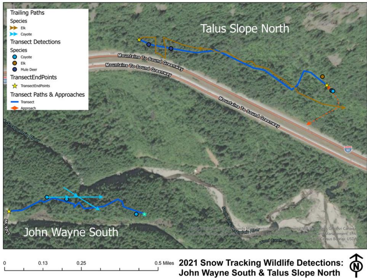
Talus Slope North & John Wayne South Transects: (Map A7)
